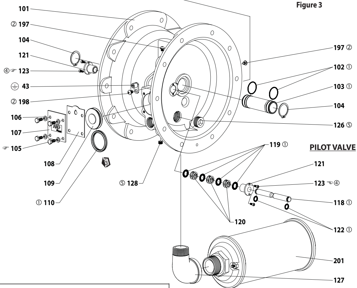
MAJOR VALVE See cross section detail, figure 4.
